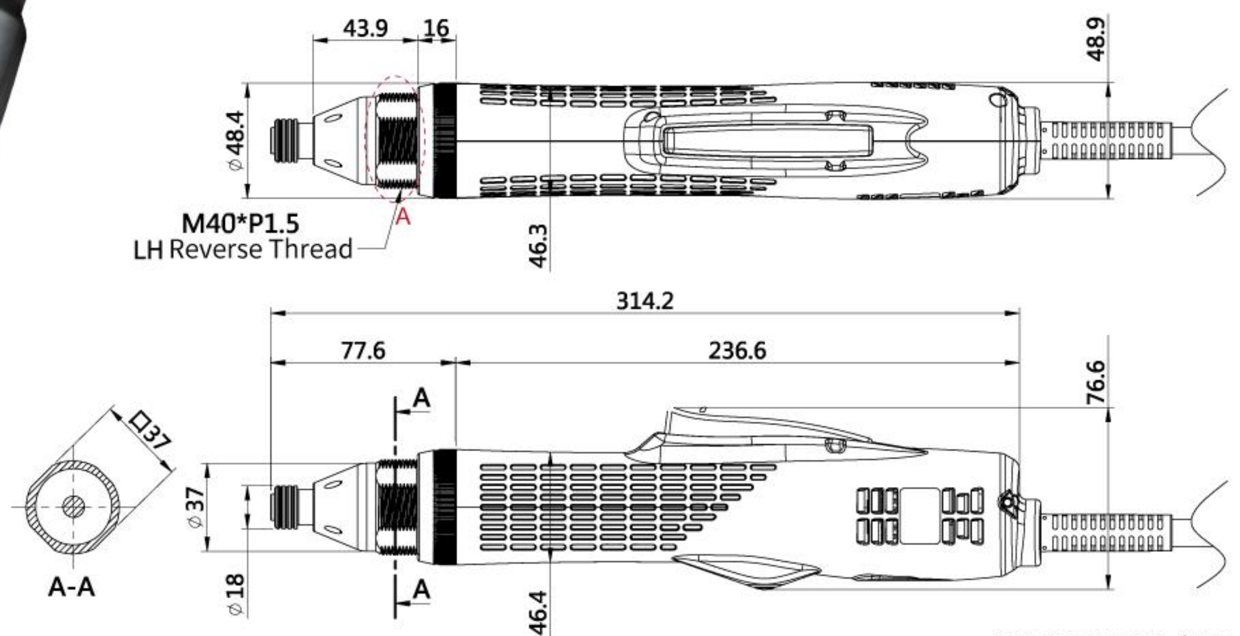
MY-SAVER 12 / 18 Unit: mm
